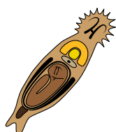
Flukes Gyrodactylus.
